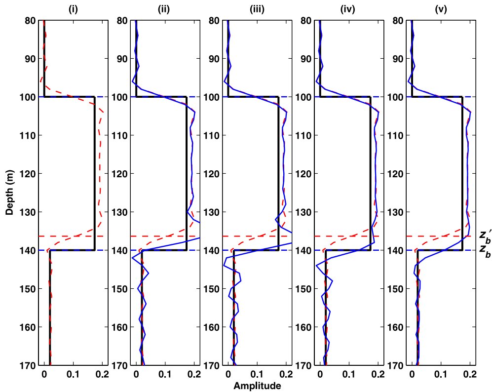
Figure 24. The cumulative sum of five terms in the leading order imaging subseries. The solid black curve shows the perturbation \alpha and the red curve shows the first approximation to \alpha or the first term in the inverse series, \alpha_1 . The blue curve shows the cumulative sum of the imaging subseries terms; e.g. in panel (ii) the sum of two terms in the subseries is shown and in panel (v) the sum of five terms in the subseries is displayed.
