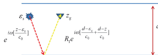
Figure 15. Use of a primary to find an image. Downgoing wave that starts at z = \epsilon_s at t = t_0 = 0 .
