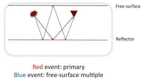
Figure 7. Case 2: a primary and a free-surface multiple (recorded data).
