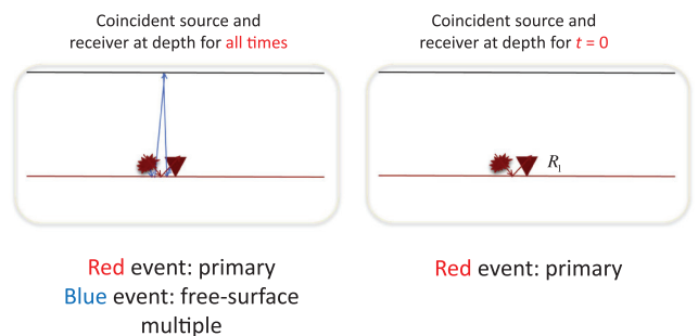
Figure 8. Case 2: a primary and a free-surface multiple. Above the reflector (predicted experiment at depth).
