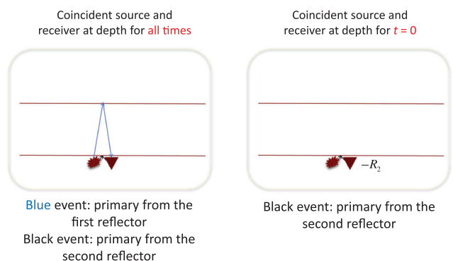
Figure 14. Case 3: two primaries and an internal multiple. Below the second reflector (predicted experiment at depth).
