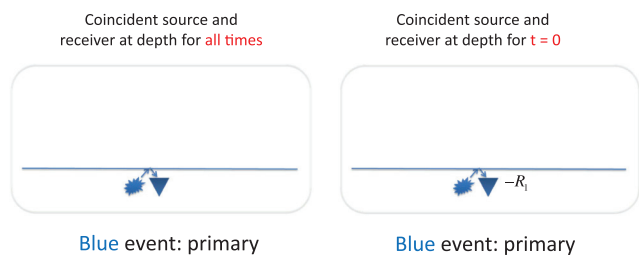
Figure 6. Case 1: a primary from a single reflector. Below the reflector (predicted experiment at depth).
