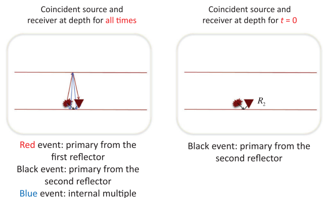
Figure 13. Case 3: two primaries and an internal multiple. Above the second reflector (predicted experiment at depth).
