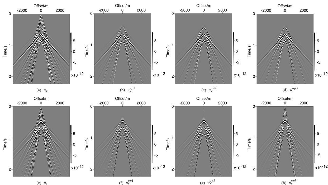
Figure 6: Wave separation on vacuum/earth model. (a) for x component total wave; (b) for x component separated up wave from case 1; (c) for x component result from case 2; (d) for x component result from case 3; (e–h) for corresponding z component results.
