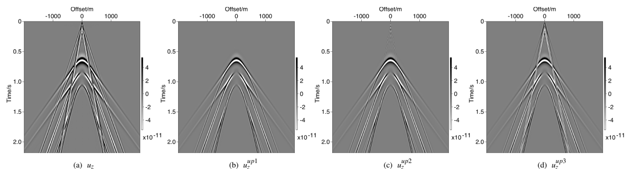
Figure 7: Wave separation on air/earth model for z component. (a) for total wave; (b) for separated up wave from case 1; (c) for the result from case 2; (d) for the result from case 3.
