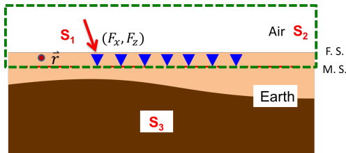
Figure 3: Three sources act on the reference medium, and the surface integral will extract the contributions from S_3 , for evaluation point \vec{r} inside the volume.
