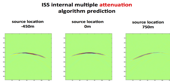
Figure 3: ISS internal multiple attenuation algorithm prediction
